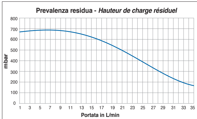
Art. 15200 NOVAHEAT 130 - DN20
